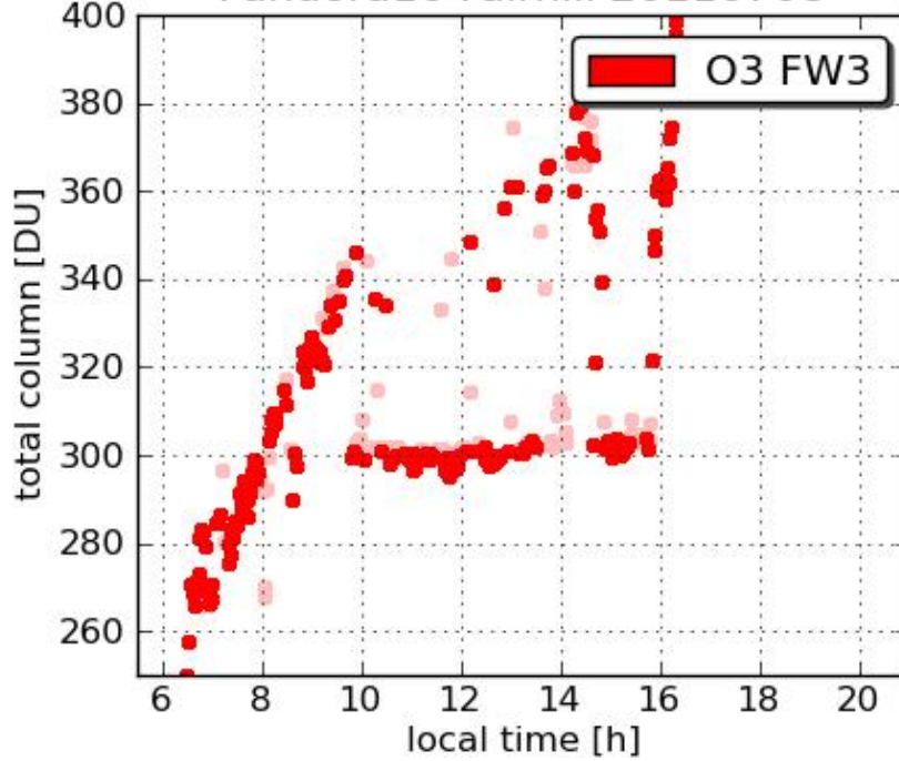
Pandora16 Fairhill 20110708
