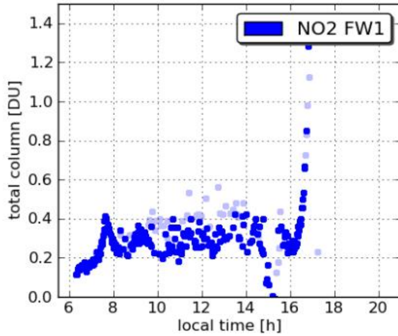
Pandora16 Fairhill 20110708
