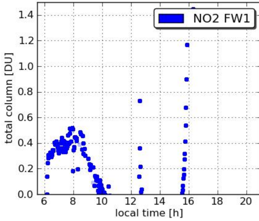
Pandora2 UMBC 20110708
