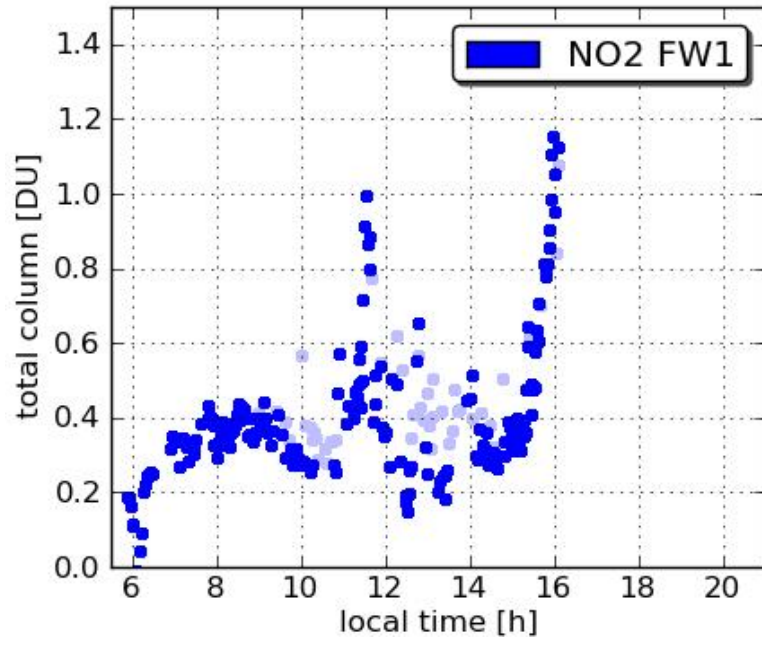
Pandora3 GSFC 20110708
