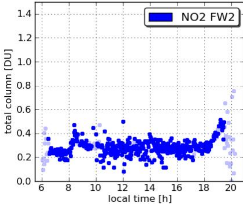
Pandora7 SERC 20110723
