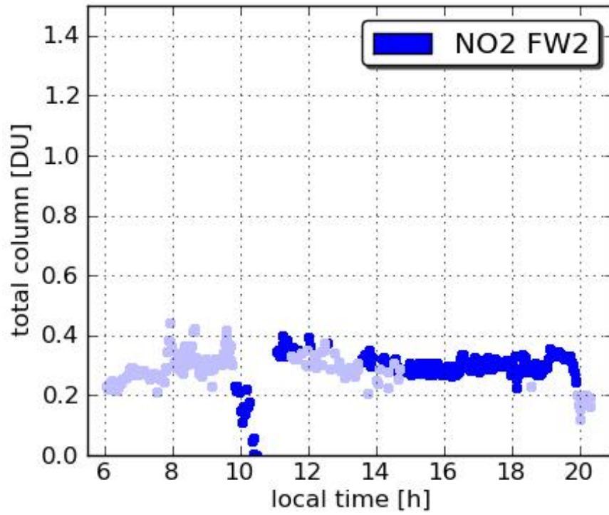
Pandora2 UMBC 20110723
