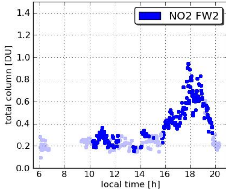
Pandora19 Essex 20110723
