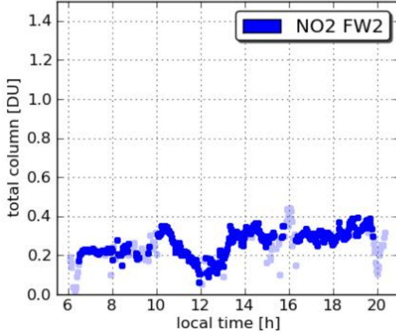
Pandora3 GSFC 20110723
