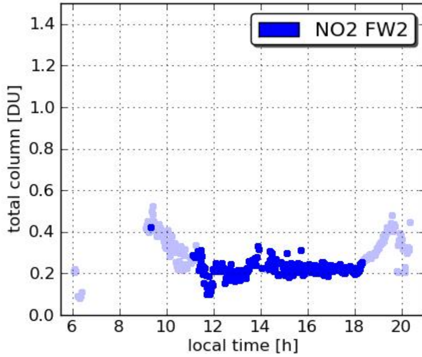
Pandora16 Fairhill 20110723
