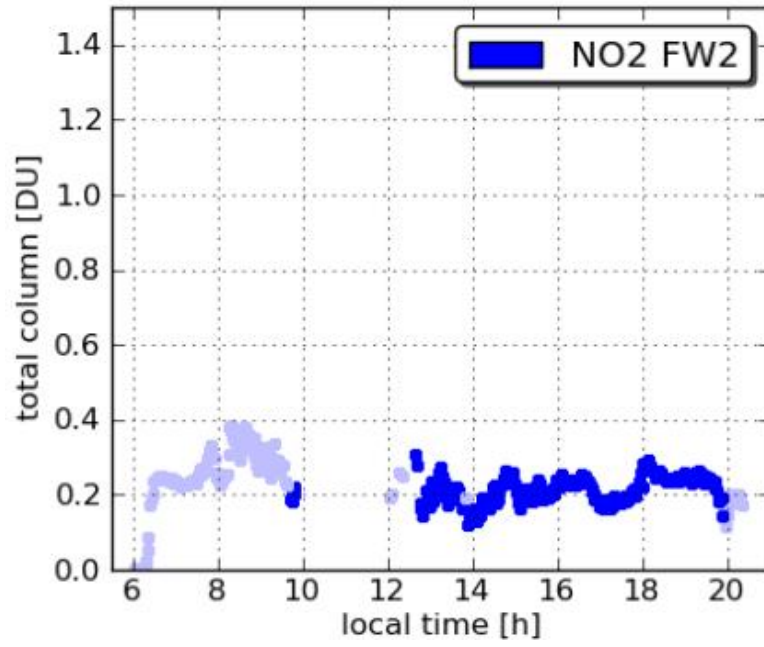
Pandora17 Padonia 20110723
