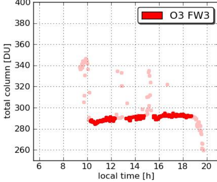
Pandora19 Essex 20110723
