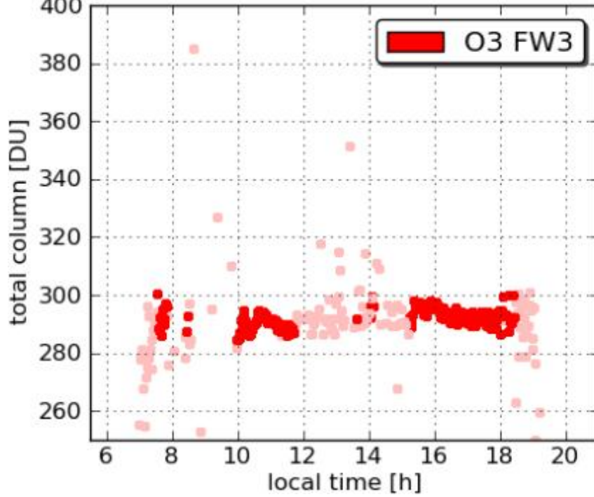
Pandora9 Oldtown 20110723
