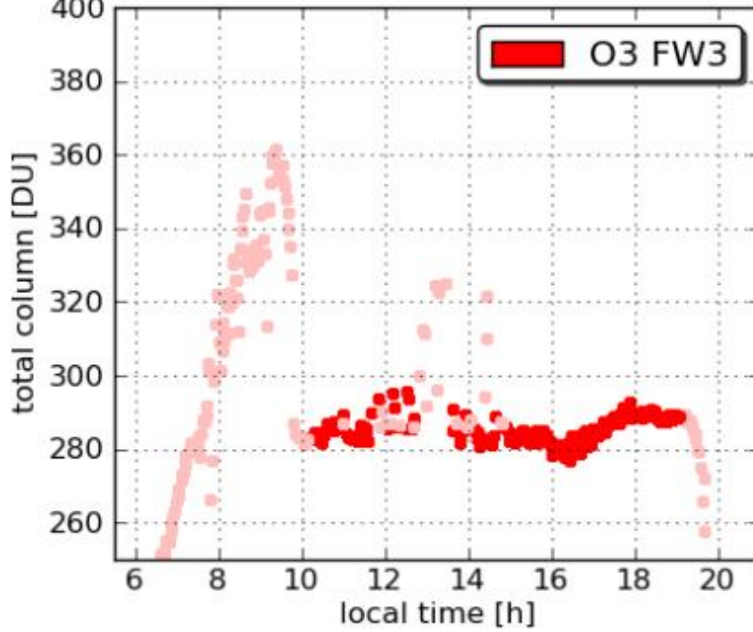
Pandora2 UMBC 20110723
