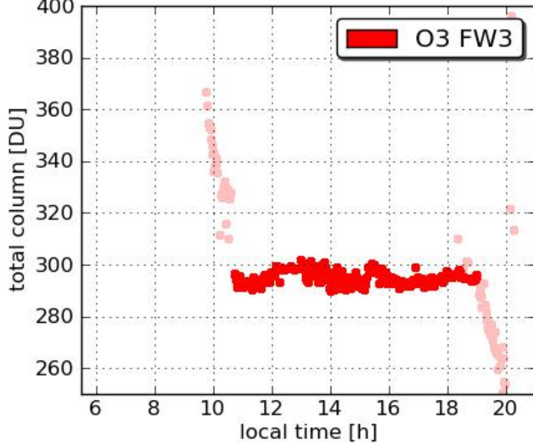
Pandora23 Aldino 20110723
