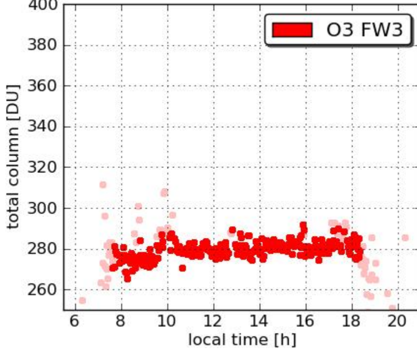
Pandora7 SERC 20110723
