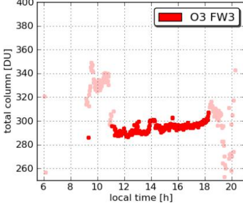
Pandora16 Fairhill 20110723
