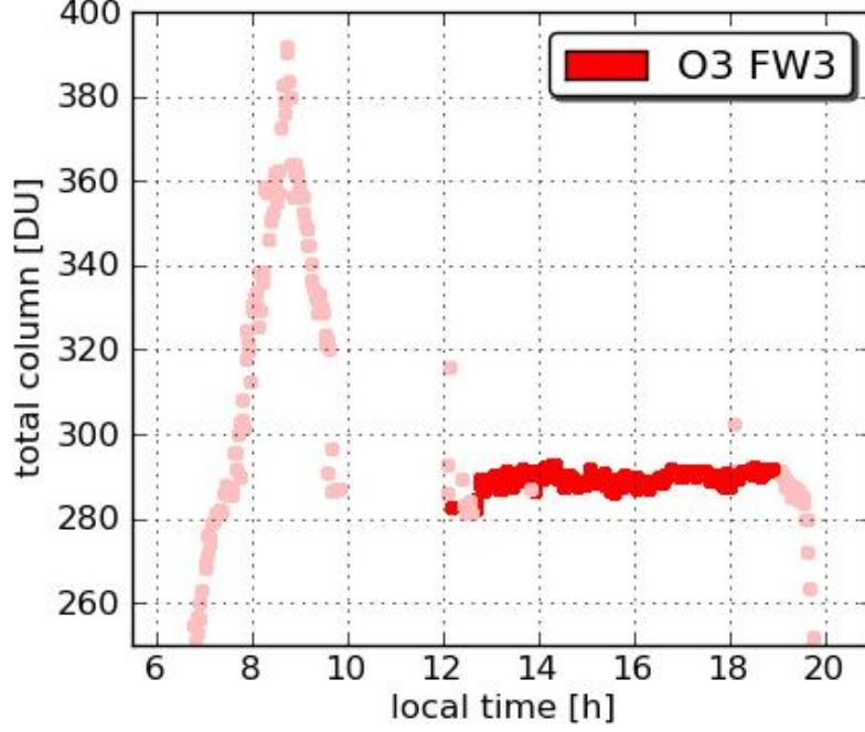
Pandora17 Padonia 20110723
