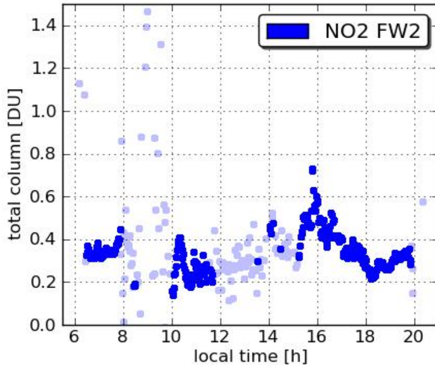
Pandora9 Oldtown 20110723
