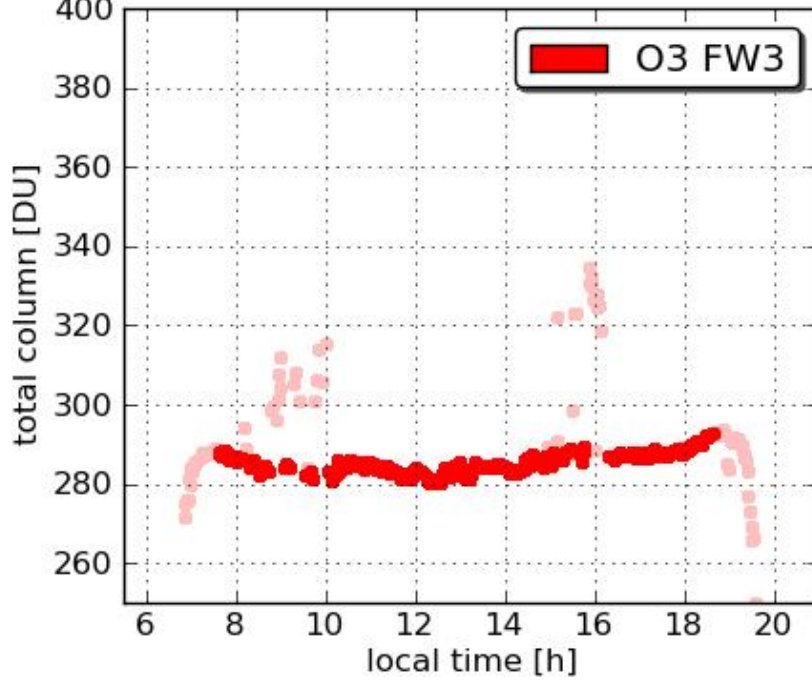
Pandora3 GSFC 20110723
