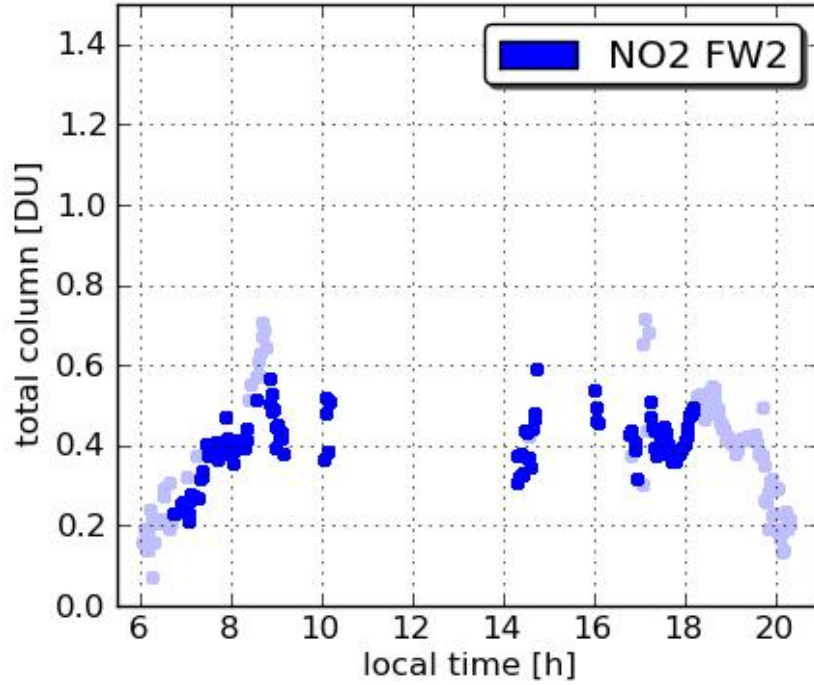
Pandora19 Essex 20110722
