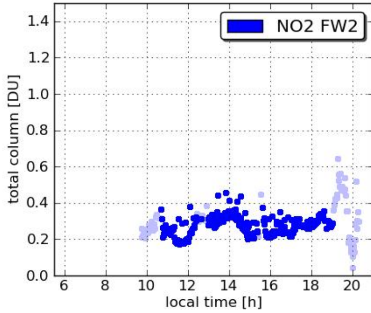
Pandora23 Aldino 20110723
