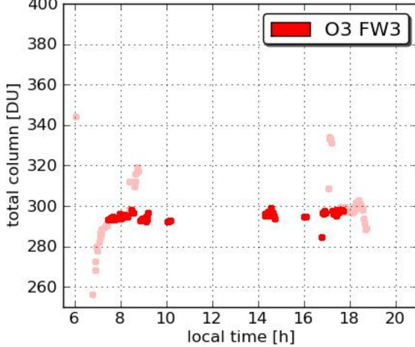
Pandora19 Essex 20110722
