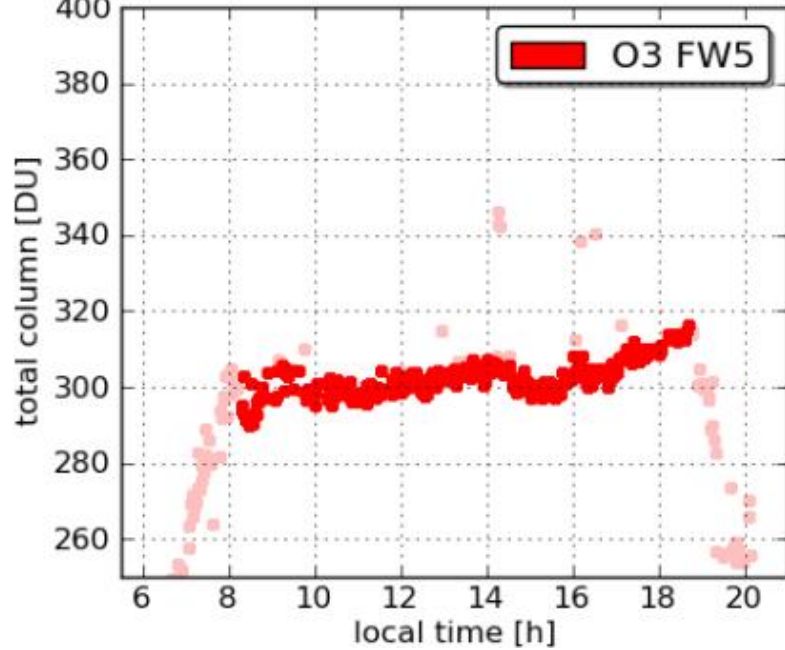
Pandora16 Fairhill 20110729
