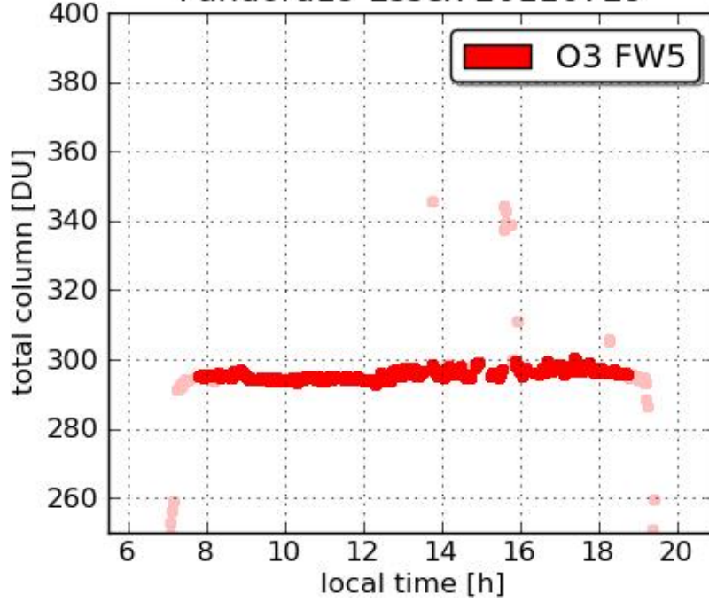
Pandora19 Essex 20110729
