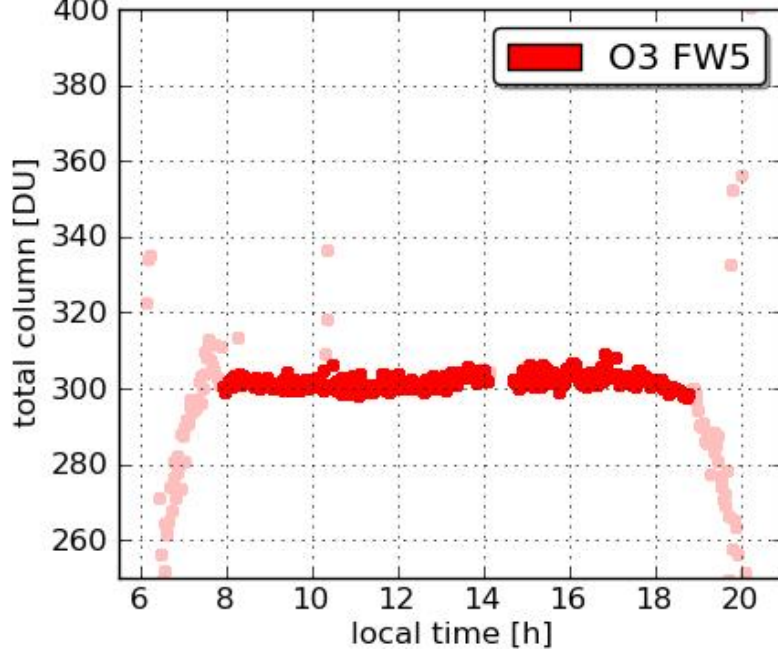
Pandora23 Aldino 20110729
