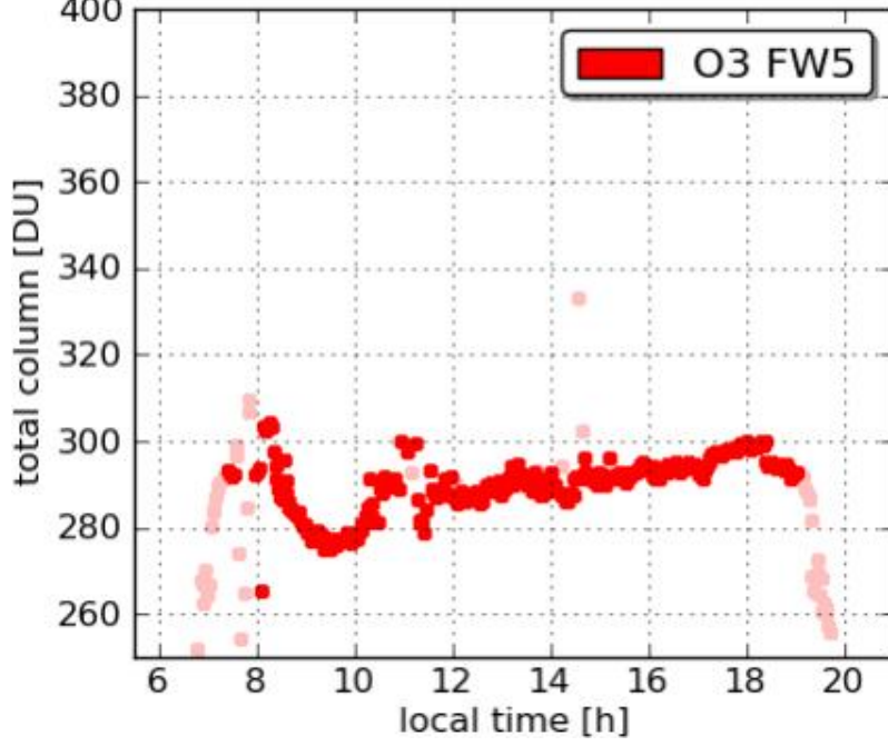
Pandora2 UMBC 20110729
