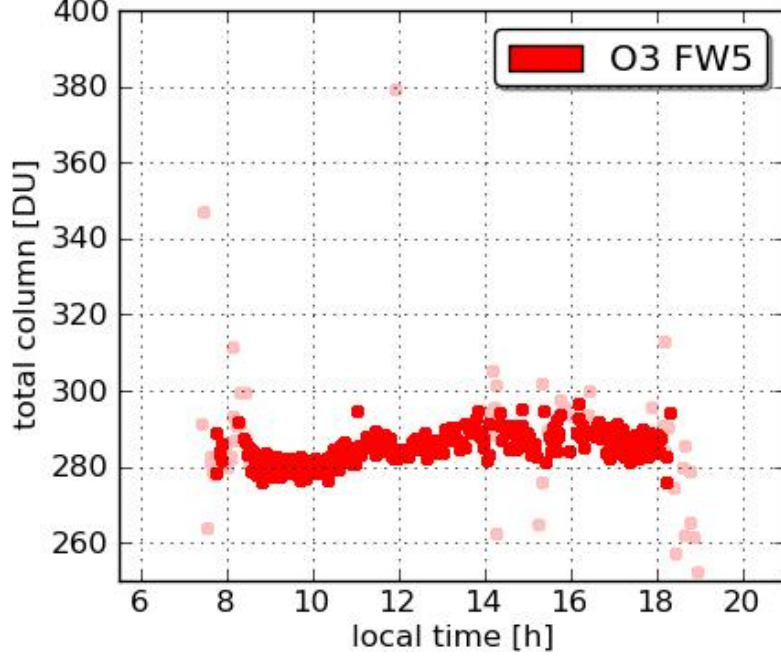
Pandora7 SERC 20110729
