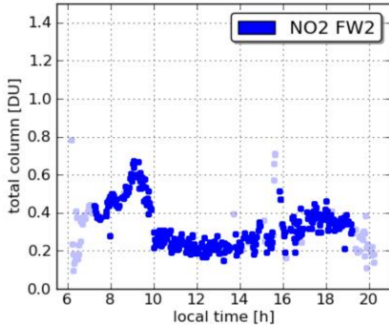
Pandora19 Essex 20110729
