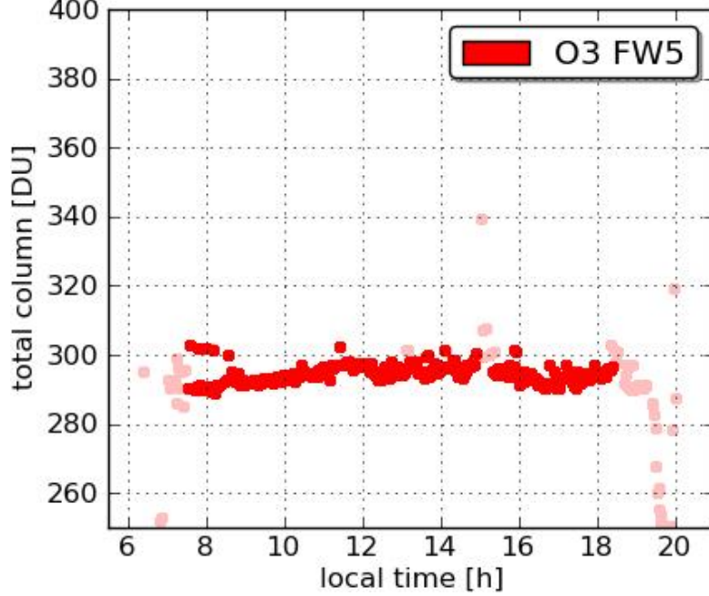
Pandora21 UMCP 20110729
