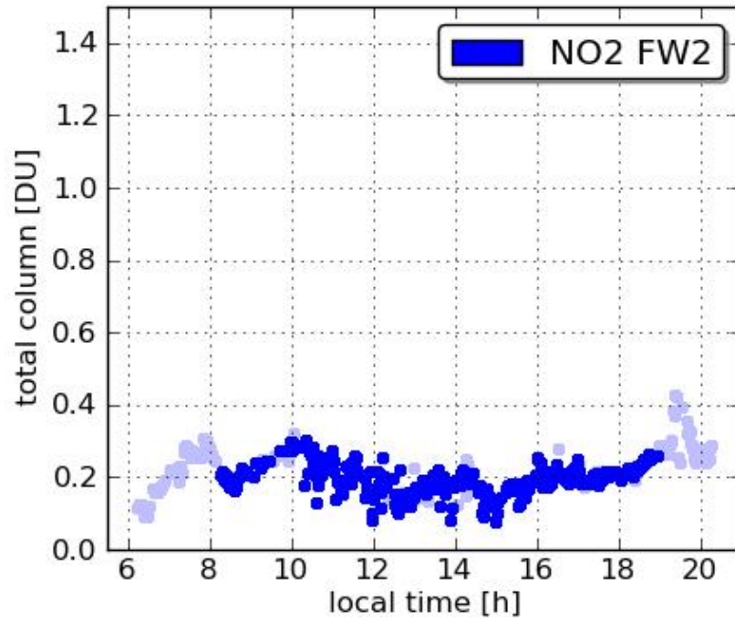
Pandora16 Fairhill 20110729
