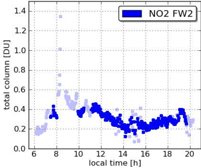
Pandora3 GSFC 20110729
