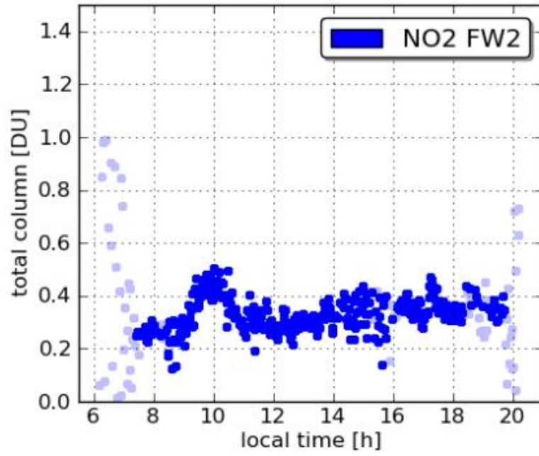
Pandora7 SERC 20110729
