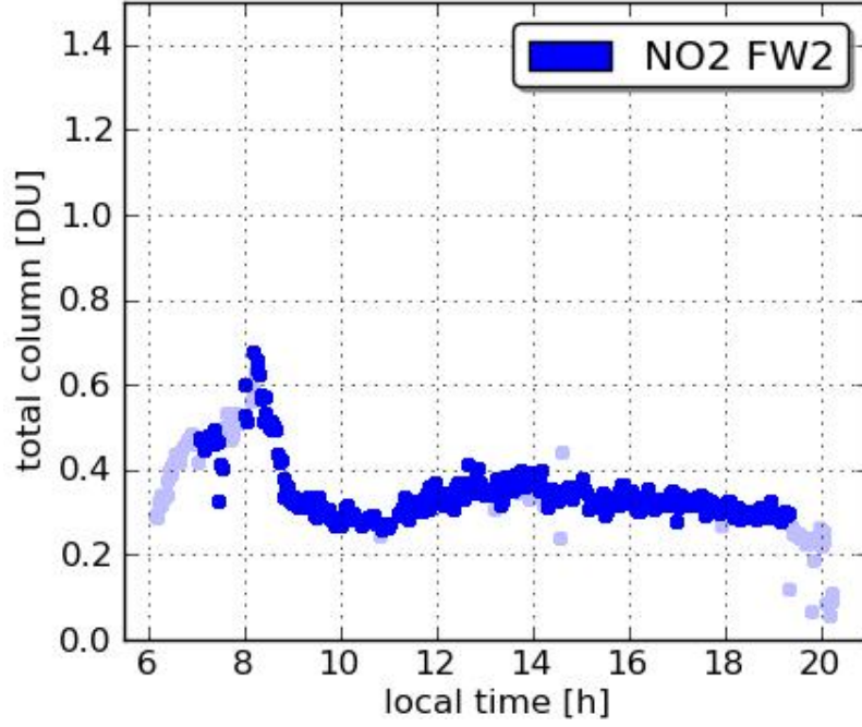
Pandora2 UMBC 20110729
