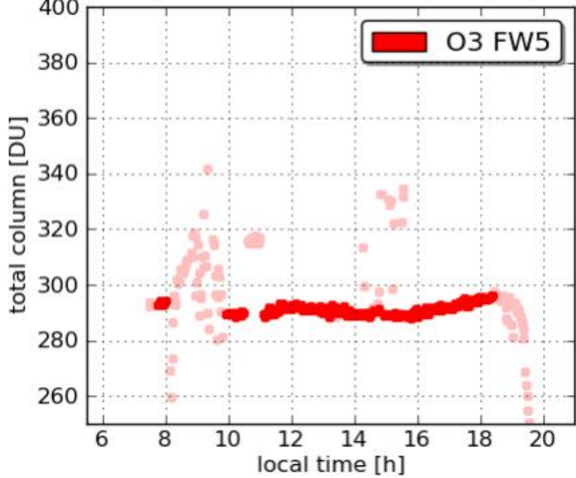
Pandora3 GSFC 20110729
