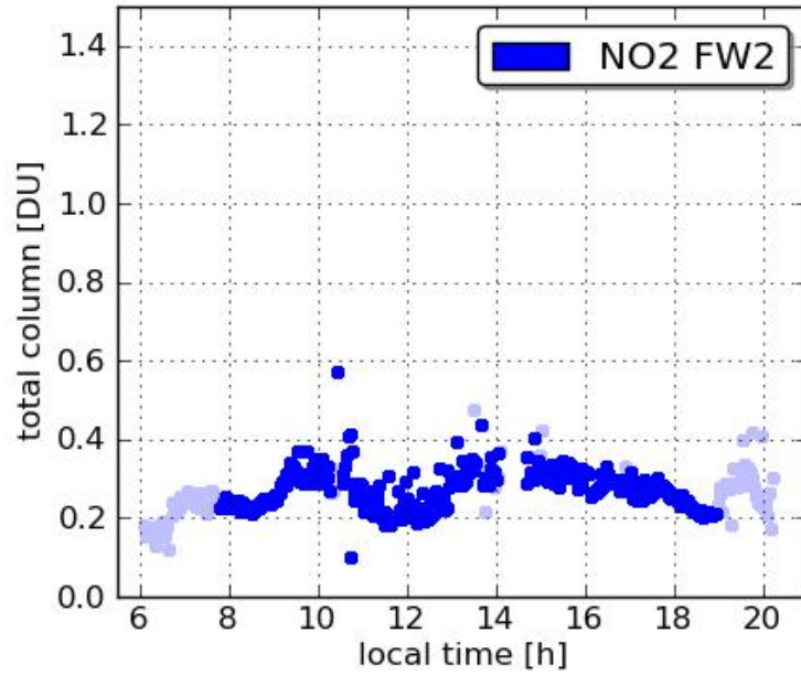
Pandora23 Aldino 20110729
