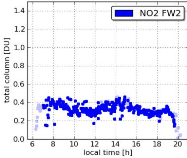
Pandora21 UMCP 20110729
