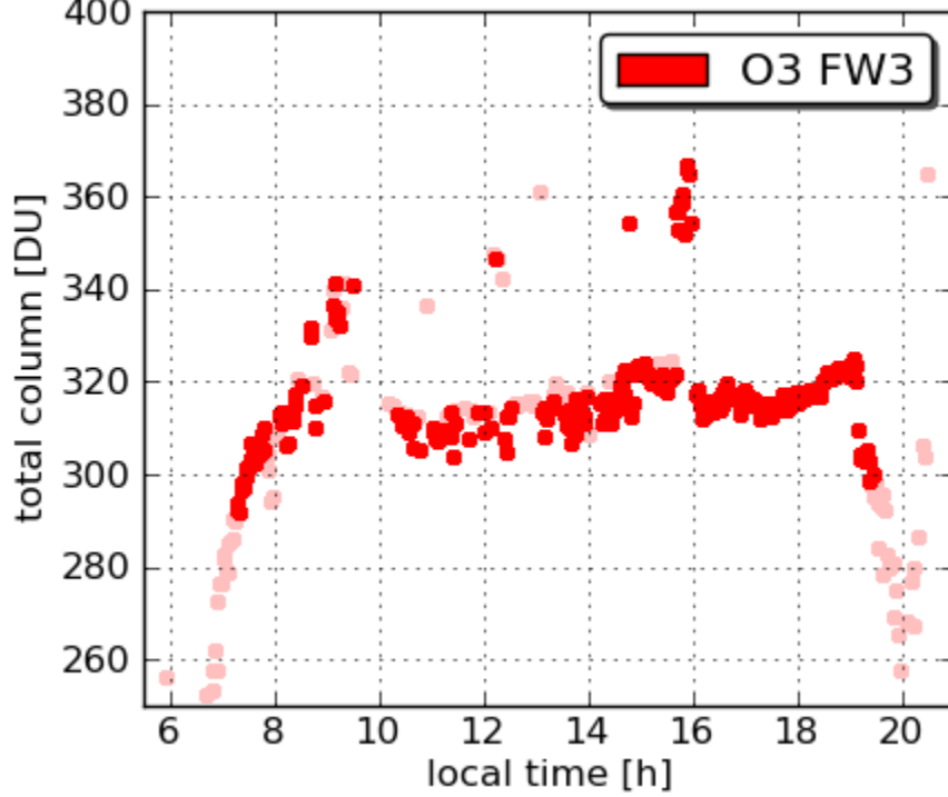
Pandora16 Fairhill 20110703
