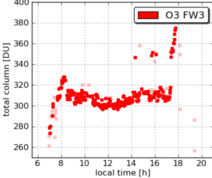
Pandora20 Beltsville 20110703
