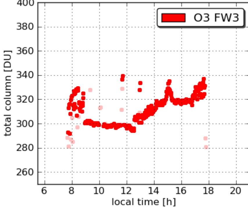
Pandora18 Edgewood 20110703
