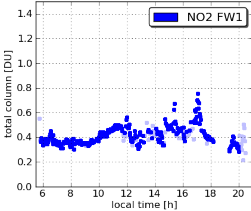
Pandora23 Aldino 20110703
