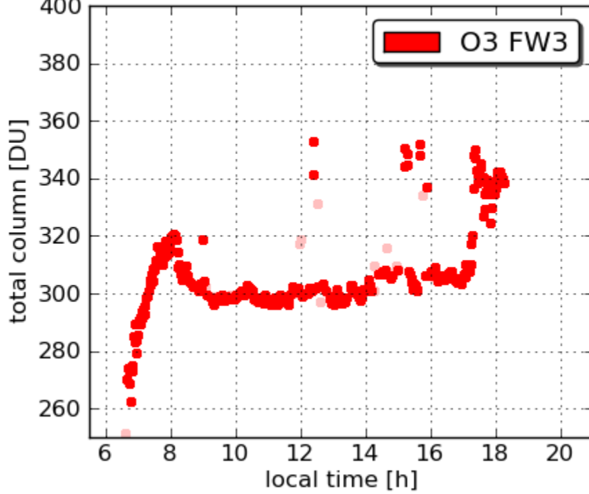
Pandora17 Padonia 20110703
