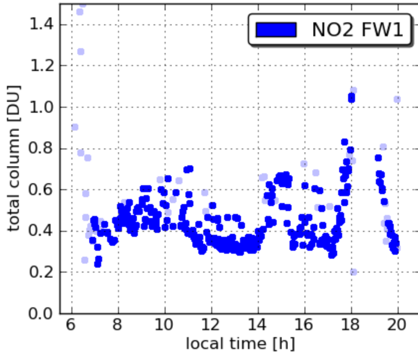
Pandora20 Beltsville 20110703
