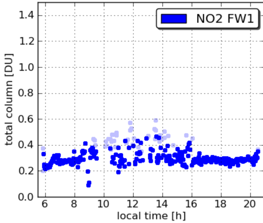
Pandora16 Fairhill 20110703
