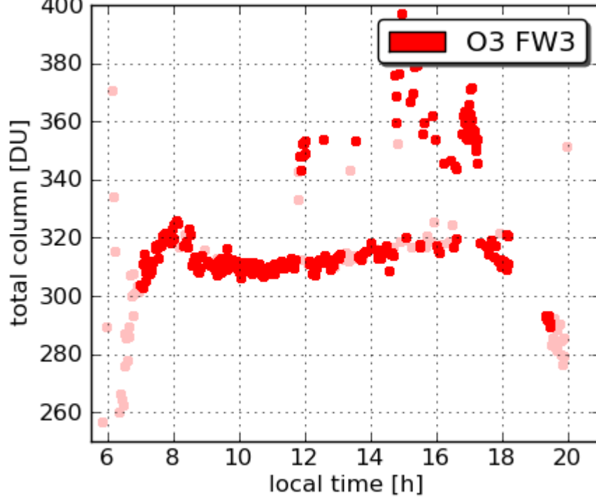
Pandora23 Aldino 20110703
