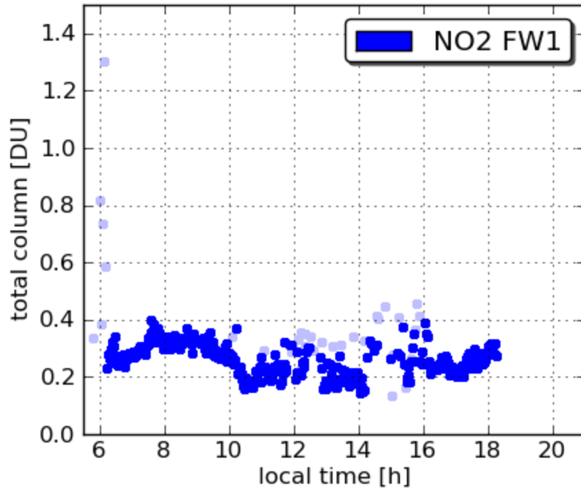
Pandora17 Padonia 20110703
