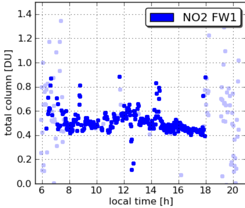
Pandora18 Edgewood 20110703
