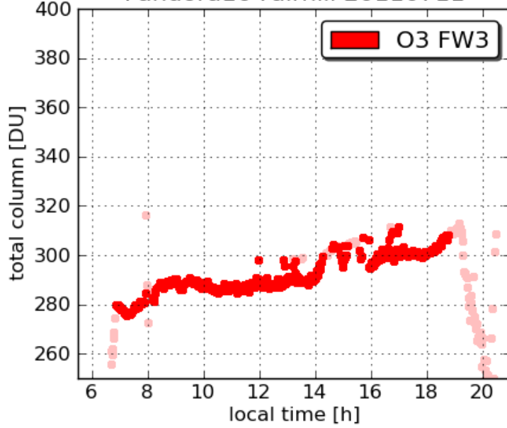
Pandora16 Fairhill 20110711
