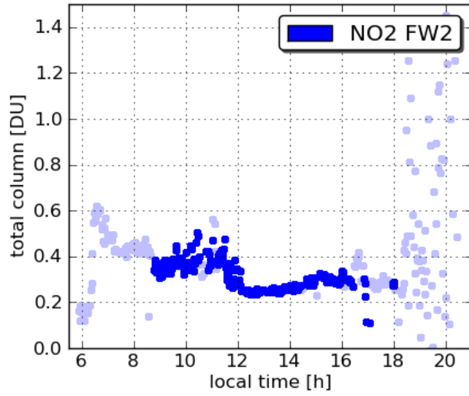
Pandora18 Edgewood 20110711
