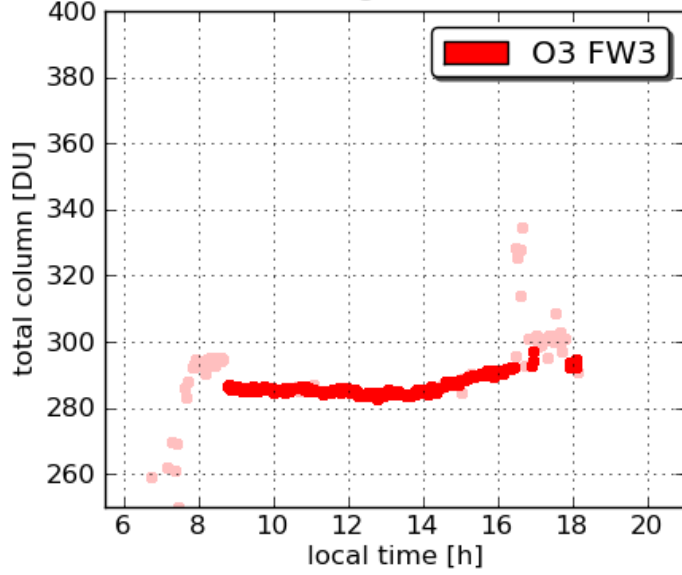
Pandora18 Edgewood 20110711
