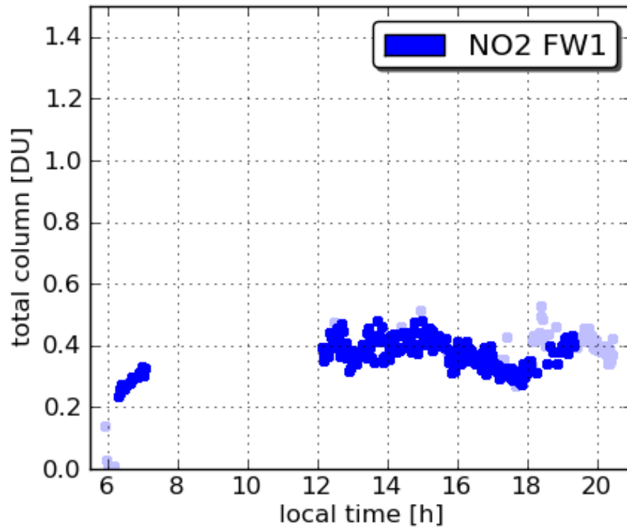
Pandora3 GSFC 20110711
