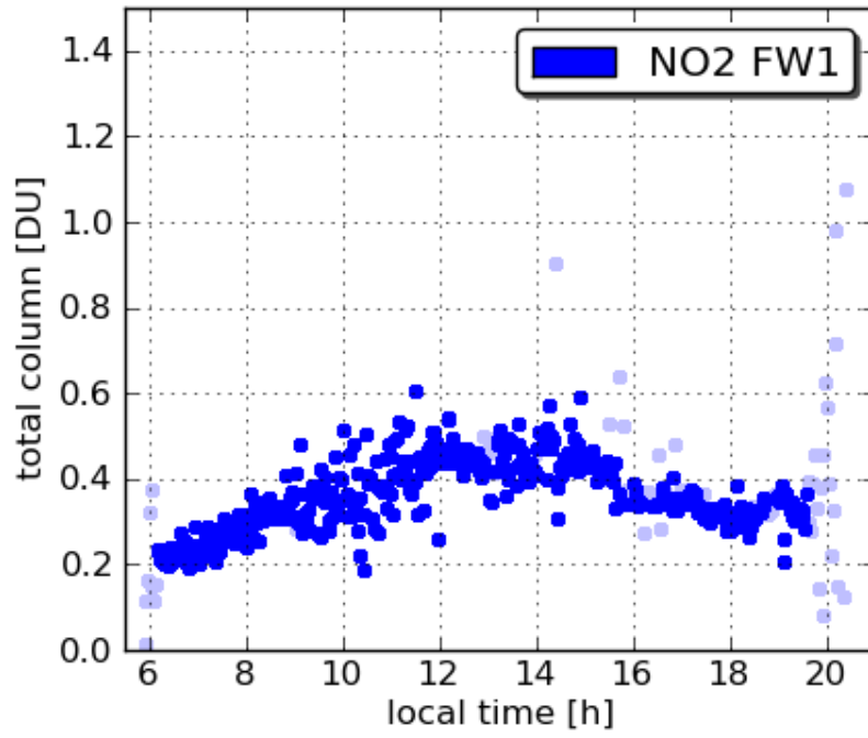
Pandora7 SERC 20110711
