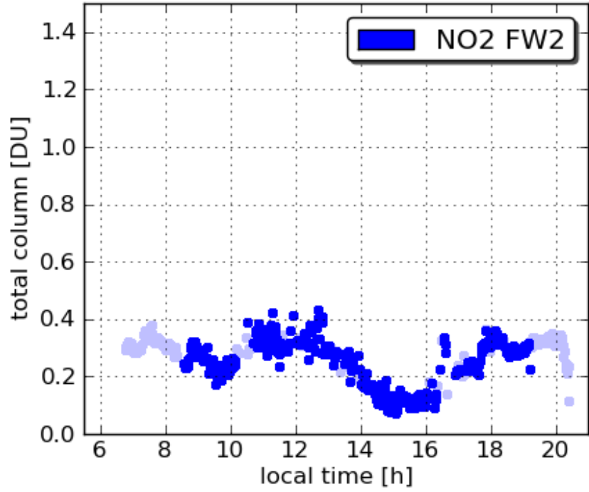
Pandora17 Padonia 20110711
