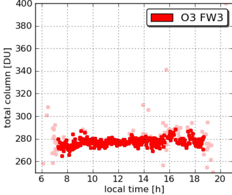
Pandora7 SERC 20110711
