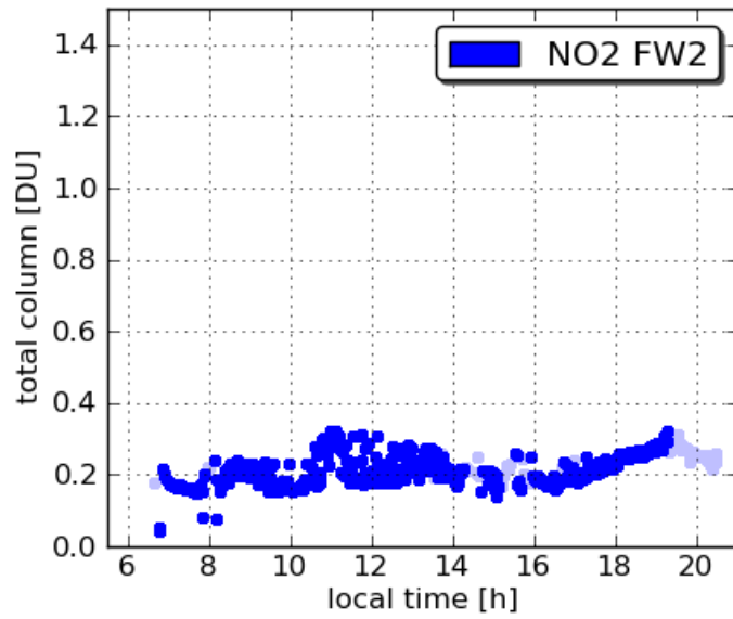
Pandora16 Fairhill 20110711
