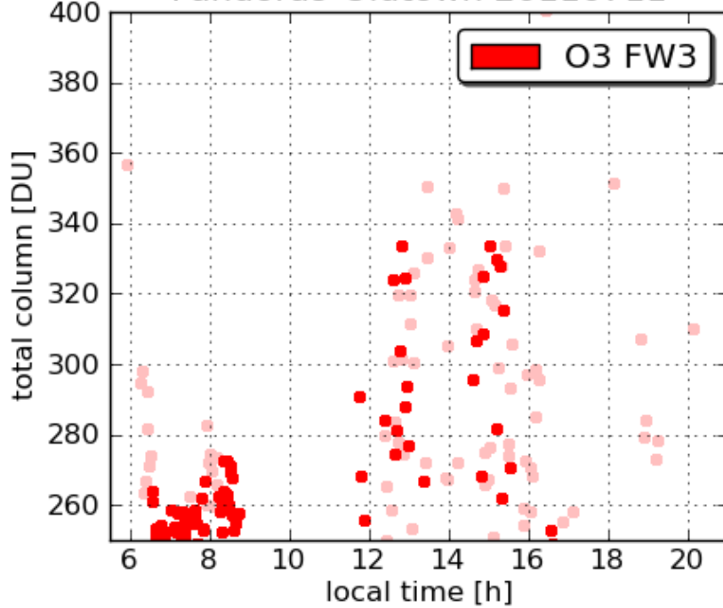
Pandora9 Oldtown 20110711
