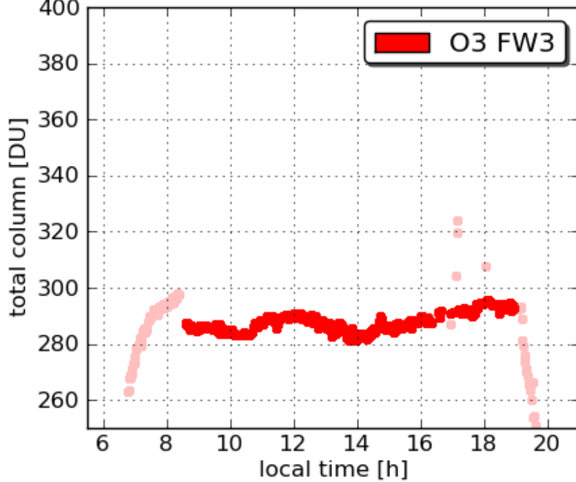
Pandora17 Padonia 20110711
