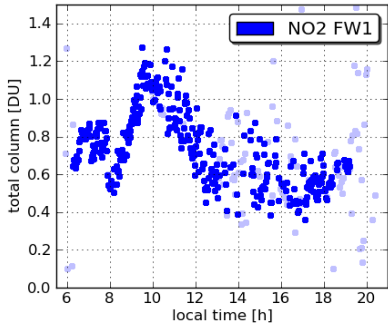
Pandora9 Oldtown 20110711
