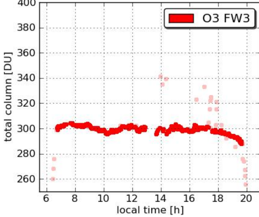
Pandora3 GSFC 20110716
