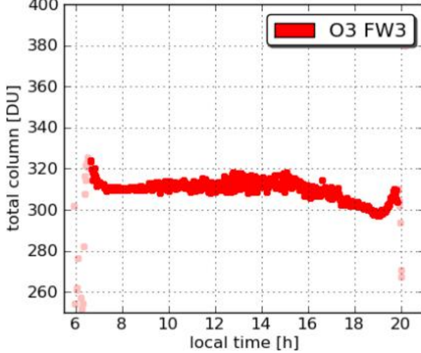
Pandora23 Aldino 20110716
