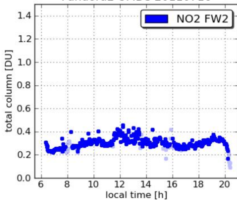
Pandora2 UMBC 20110716
