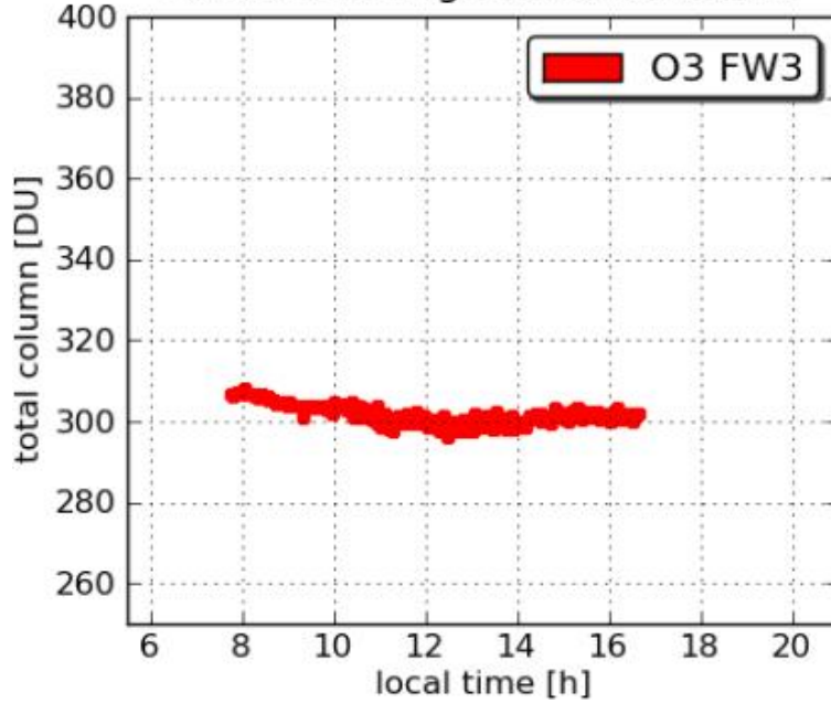
Pandora18 Edgewood 20110716
