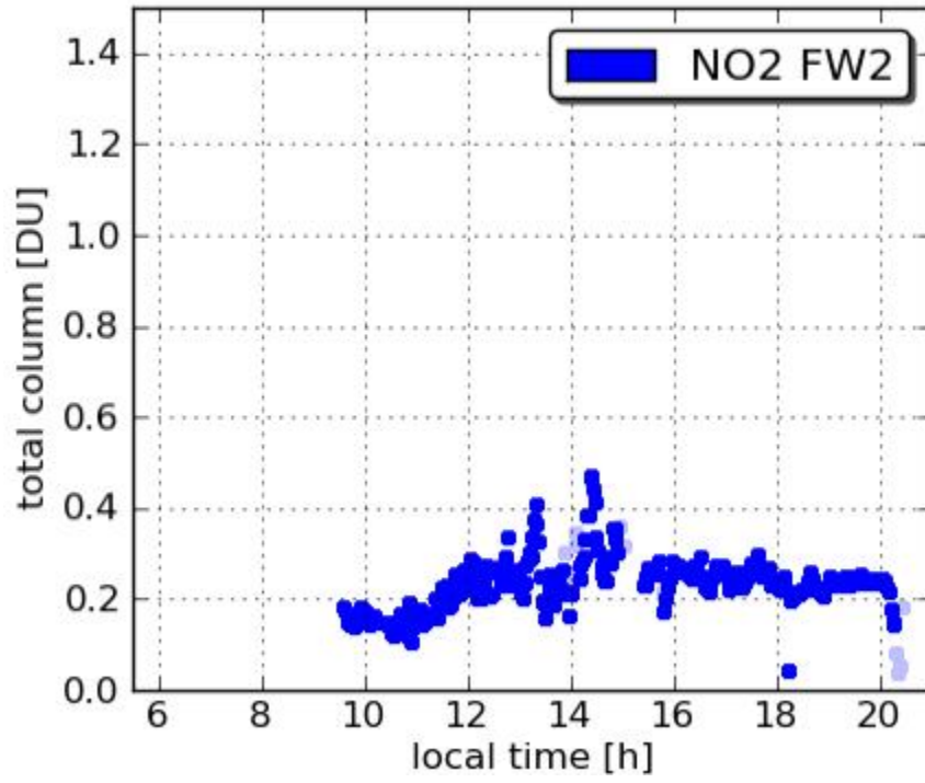
Pandora17 Padonia 20110716
