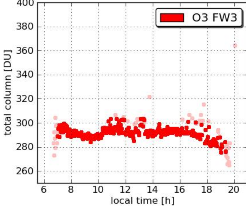
Pandora7 SERC 20110716
