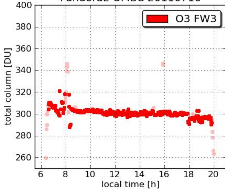
Pandora2 UMBC 20110716
