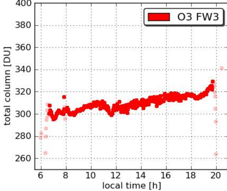
Pandora16 Fairhill 20110716
