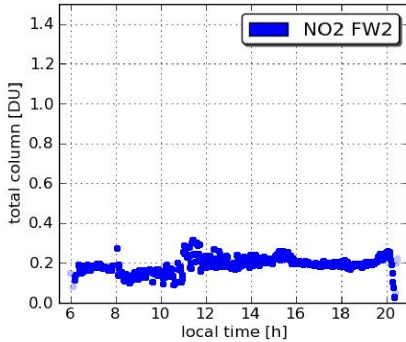
Pandora16 Fairhill 20110716
