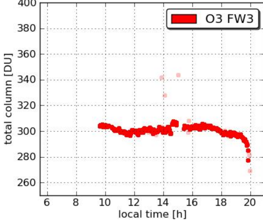
Pandora17 Padonia 20110716
