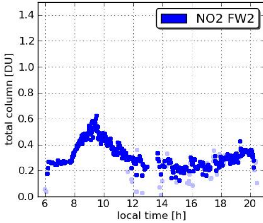
Pandora3 GSFC 20110716
