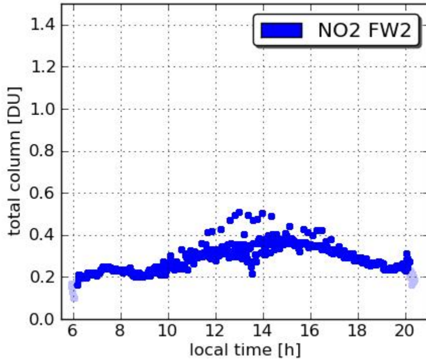
Pandora23 Aldino 20110716
