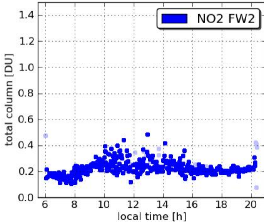
Pandora7 SERC 20110716
