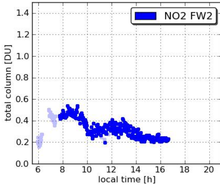
Pandora18 Edgewood 20110716
