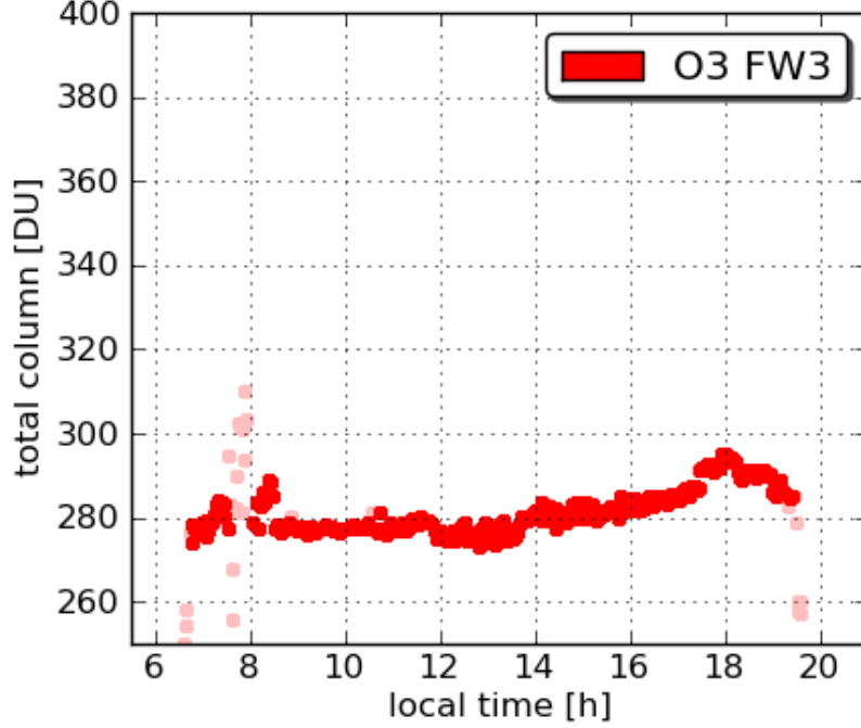
Pandora2 UMBC 20110726
