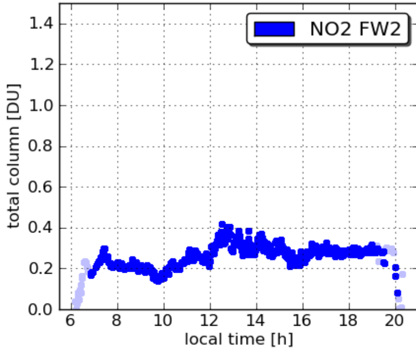
Pandora17 Padonia 20110726
