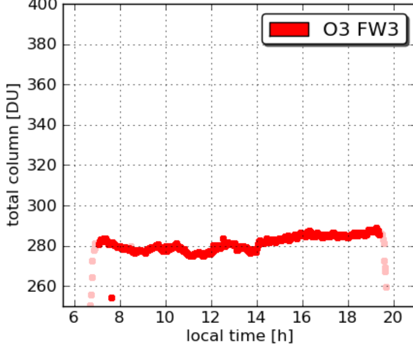
Pandora3 GSFC 20110726
