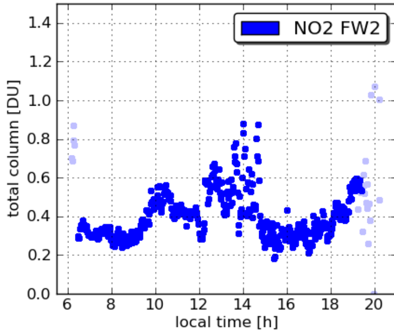
Pandora9 Oldtown 20110726
