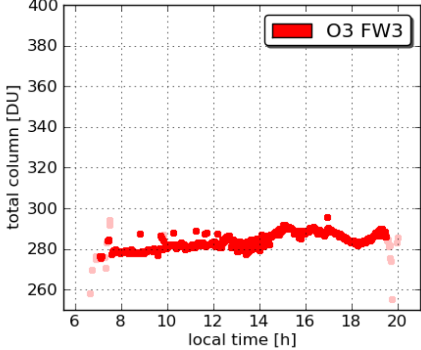
Pandora21 UMCP 20110726
