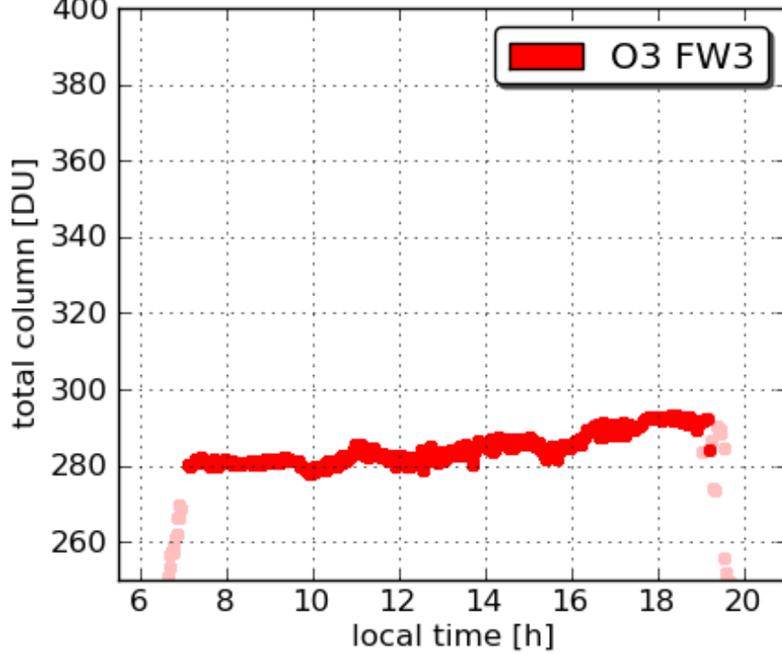
Pandora17 Padonia 20110726
