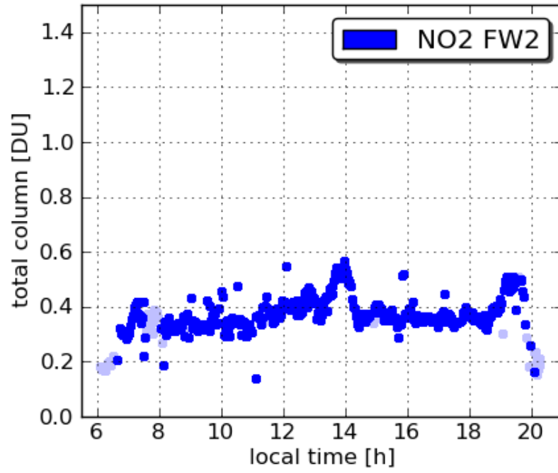
Pandora2 UMBC 20110726
