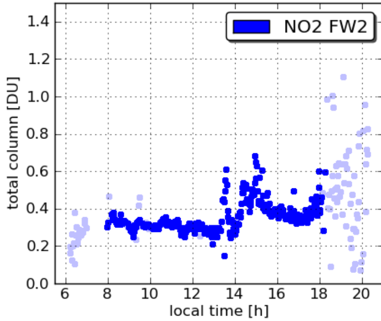
Pandora18 Edgewood 20110726
