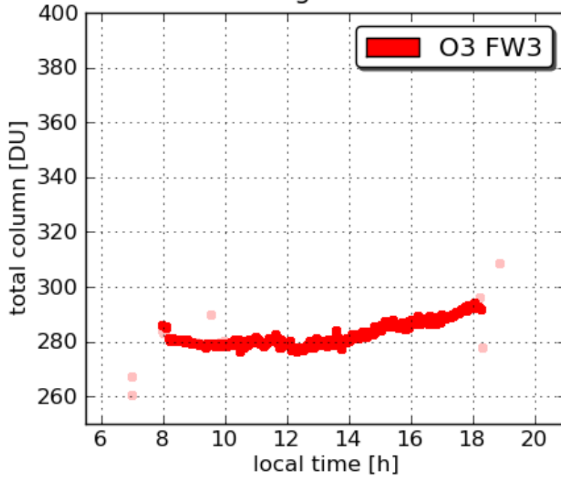
Pandora18 Edgewood 20110726
