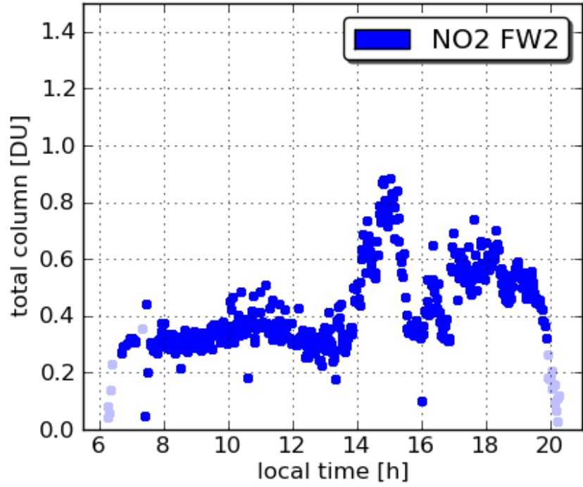
Pandora21 UMCP 20110726
