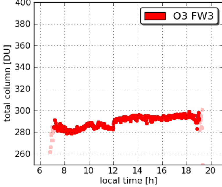
Pandora9 Oldtown 20110726
