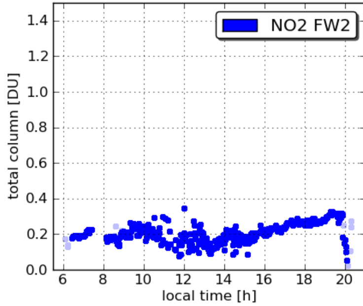
Pandora16 Fairhill 20110726
