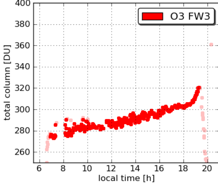
Pandora16 Fairhill 20110726
