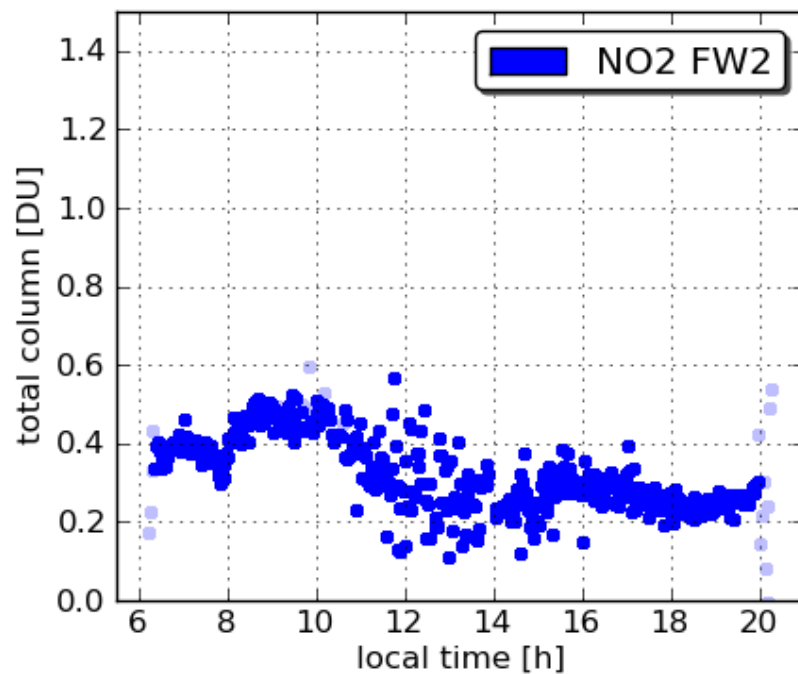
Pandora7 SERC 20110726
