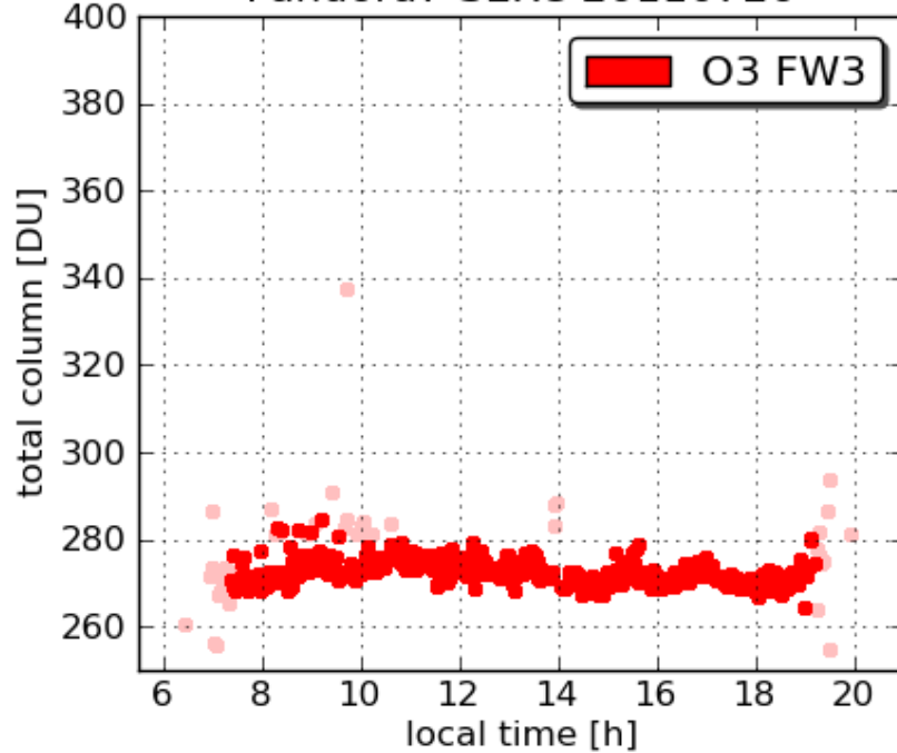
Pandora7 SERC 20110726
