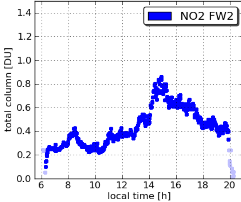
Pandora3 GSFC 20110726
