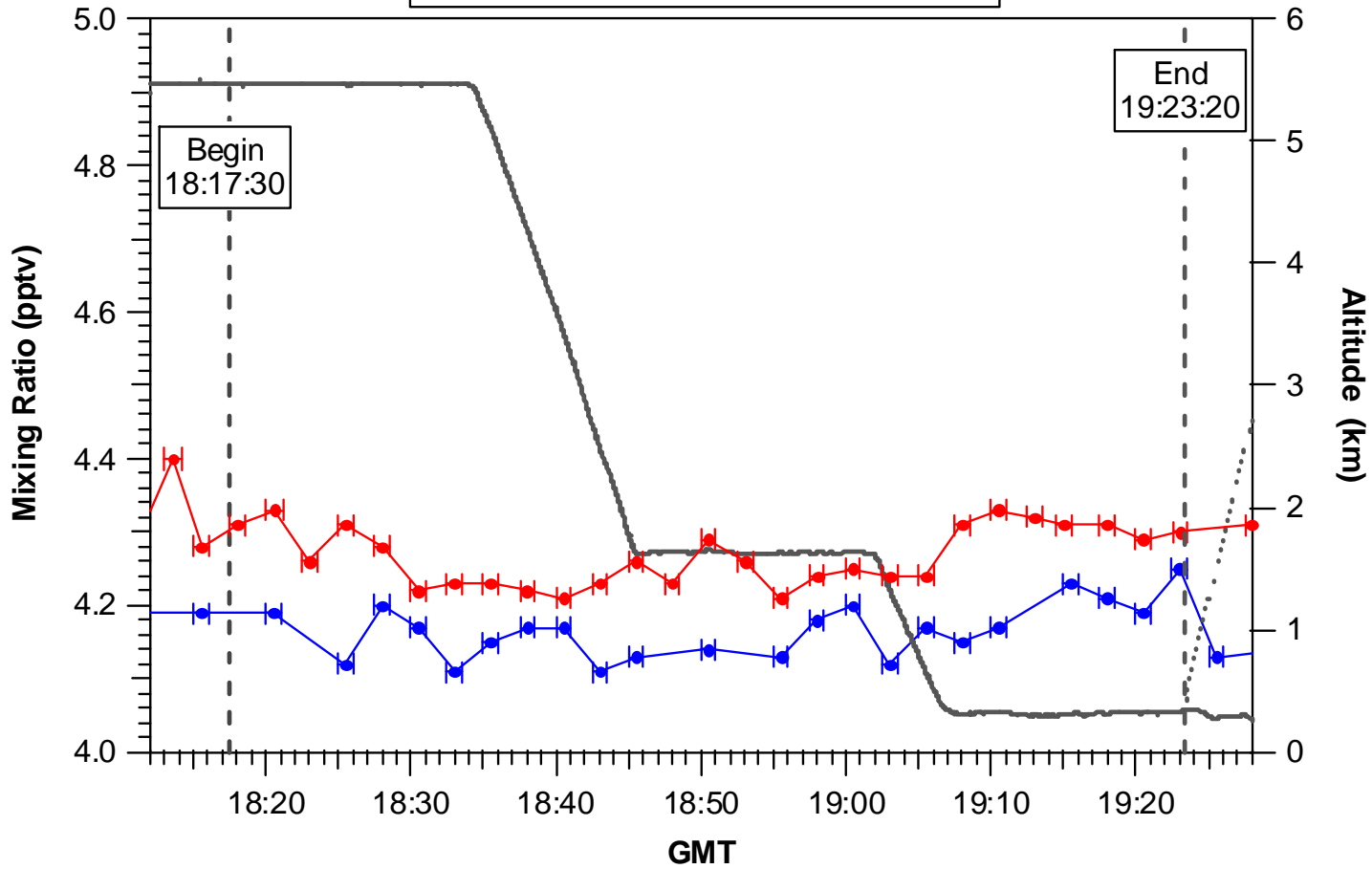
H-1211 Comparison 05/15/2006 —●— DC-8 WAS R1 —●— C-130 WAS R1
