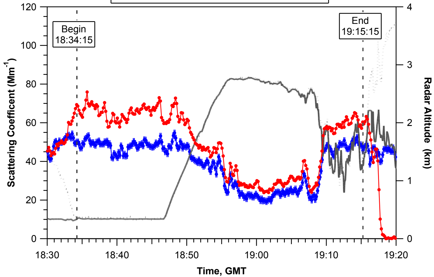
550 nm Submicron Scattering Comparison 03/19/2006
